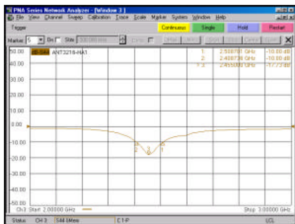
ANT3216T2450HA1
