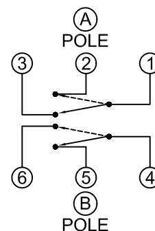
SWITCH SEQUENCE
