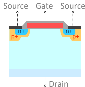
Planar MOSFET (up to 1500V, high EAS)
