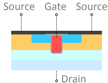
Trench MOSFET (Low R_{ch} )
