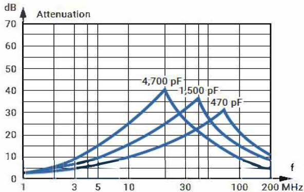
Suppression vs. Frequency, Typical Values
