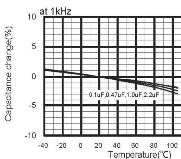
Temperature Characteristics
