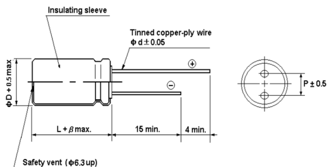
Dimensions of ΦD & L
