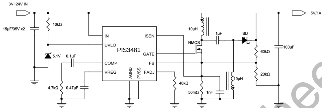
Figure8 PIS3481 Typical SEPIC Application
