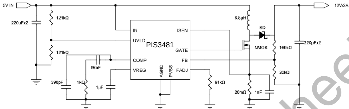
Figure 3 PIS3481 Typical Boost Application
