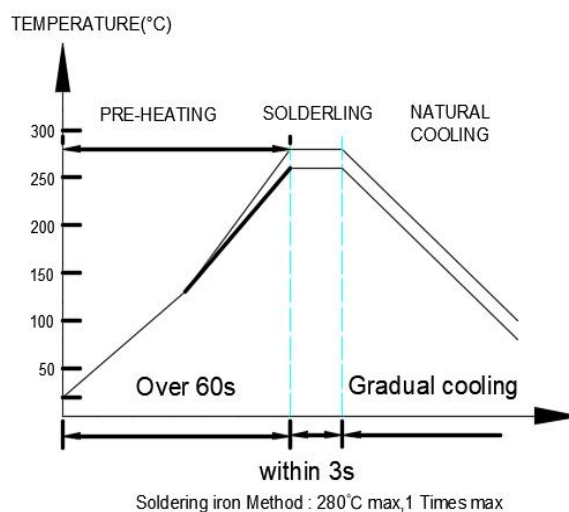
Fig.2 Iron soldering temperature profiles
