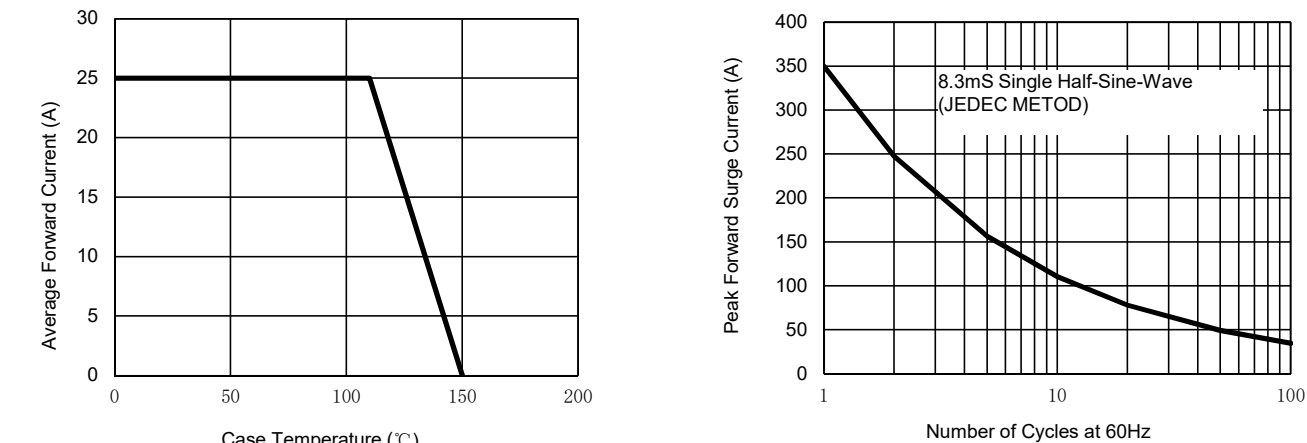
Fig. 1 - Forward Current Derating Curve
