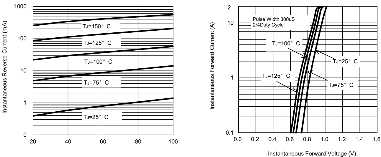
Fig. 3 - Typical Reverse Characteristics
