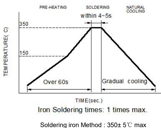
Fig.2 Iron Reflow
