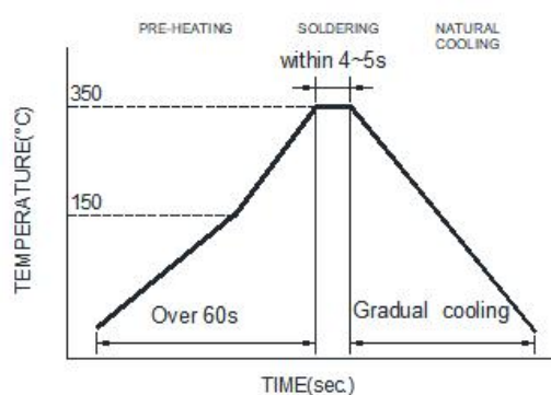
Fig.2 Iron soldering temperature profiles
