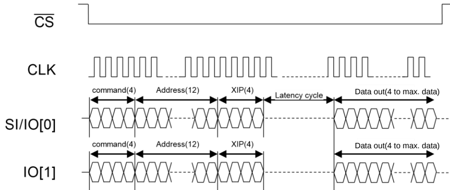
Figure 47 : Timing Description of 2-2-2 Instruction Type (Read with XIP)
