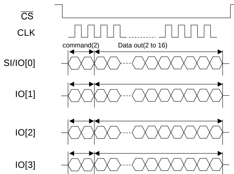
Figure 50 : Timing Description of 4-0-4 Instruction Type (Read)
