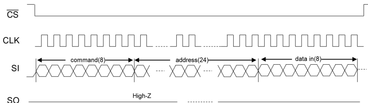
Figure 10 : Description of Write Operation (SSPI mode)
