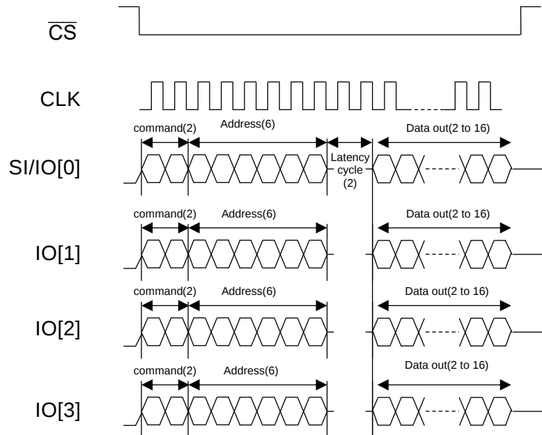
Figure 52 : Timing Description of 4-4-4 Any Register Instruction Type (Read)
