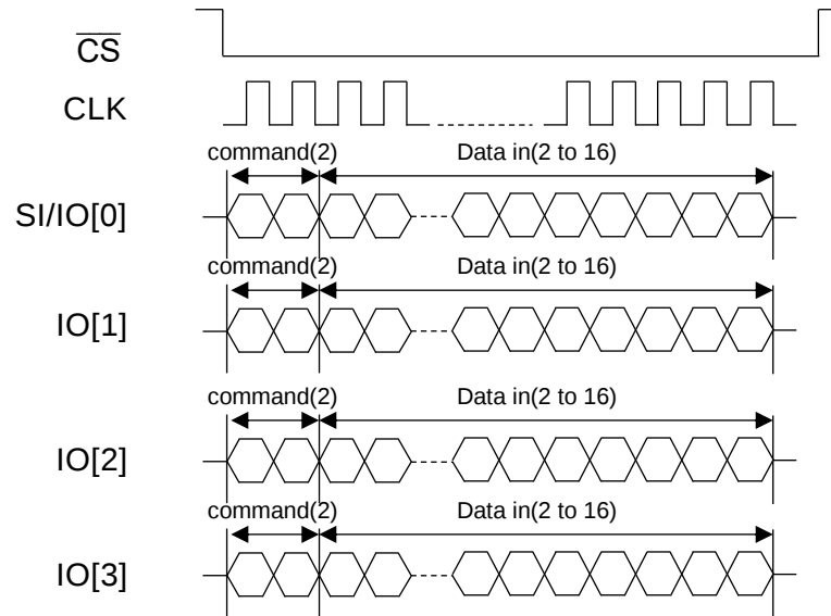
Figure 51 : Timing Description of 4-0-4 Instruction Type (Write)
