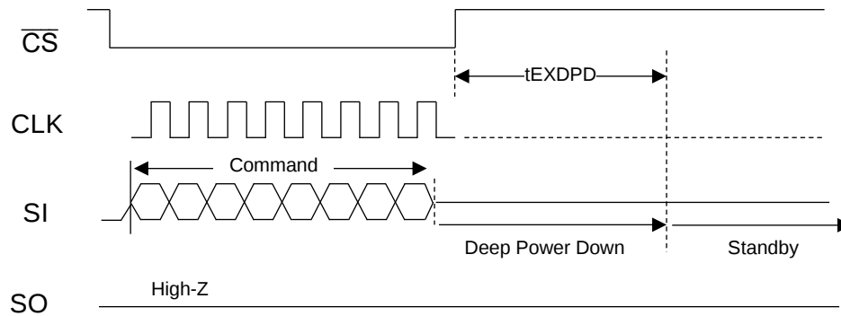
Figure 16 : Exit Deep Power Down Mode by SPI Command
