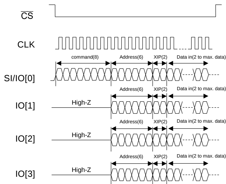
Figure 41 : Timing Description of 1-4-4 Instruction Type (Write with XIP)
