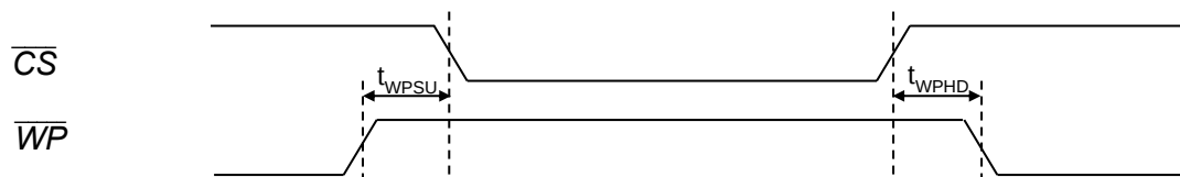
Figure 21 : \overline{WP} Operation Timing
