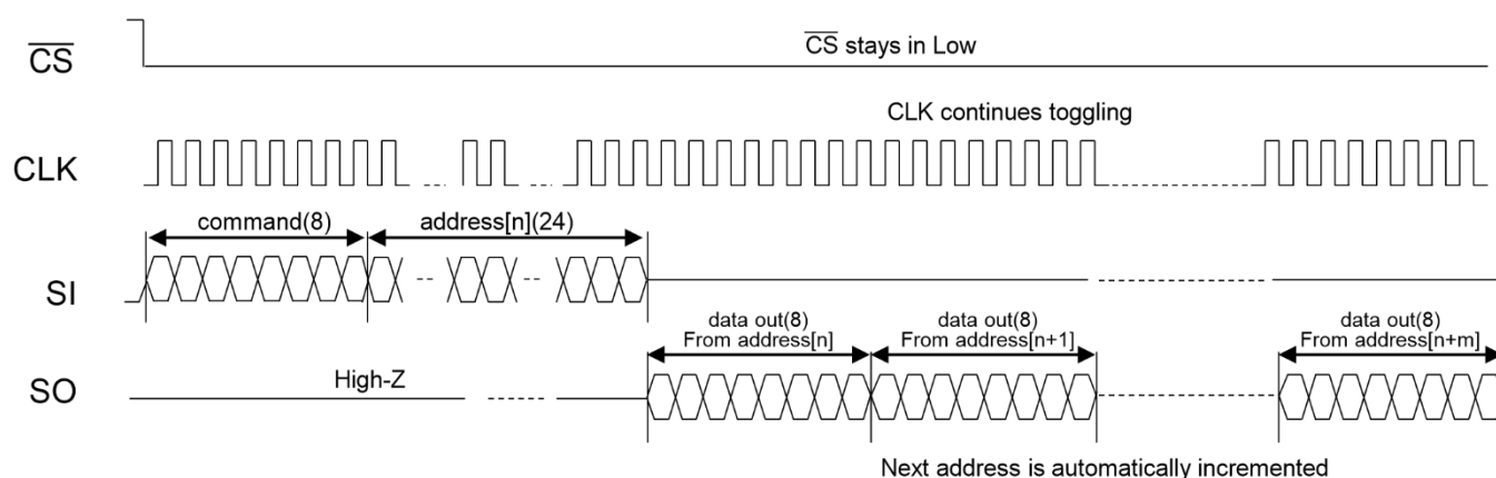
Figure 12 : Description of Continuing Read Operation (SSIP mode)
