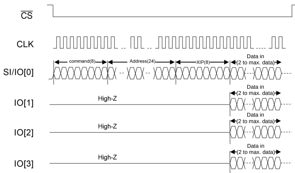
Figure 39 : Timing Description of 1-1-4 Instruction Type (Write with XIP)
