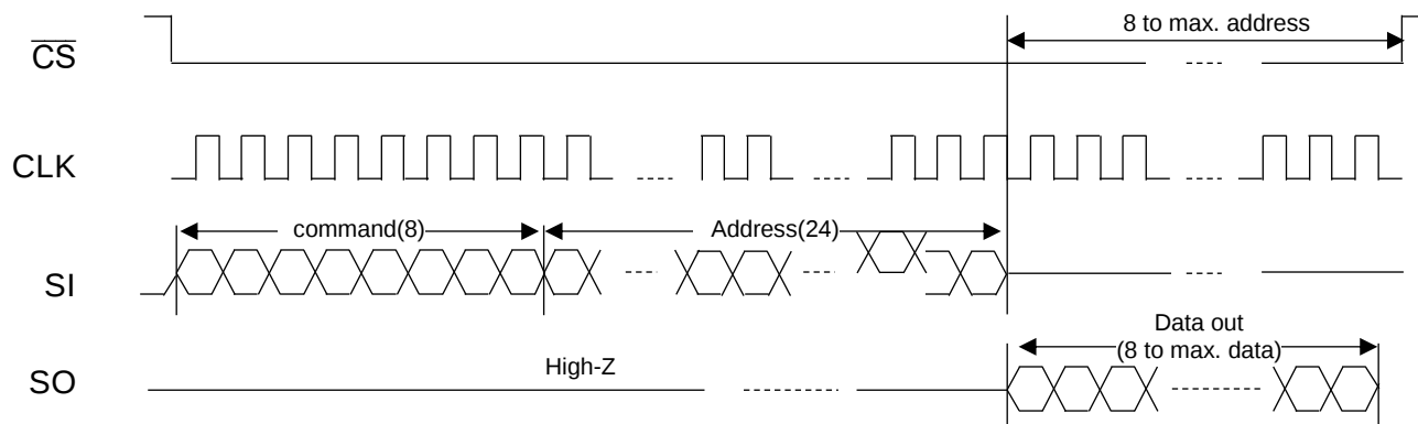
Figure 26 : Timing Description of 1-1-1 Instruction Type (Read without XIP)
