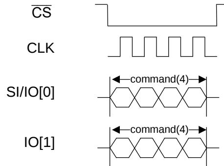
Figure 42 : Timing Description of 2-0-0 Instruction Type
