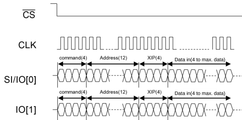
Figure 48 : Timing Description of 2-2-2 Instruction Type (Write with XIP)
