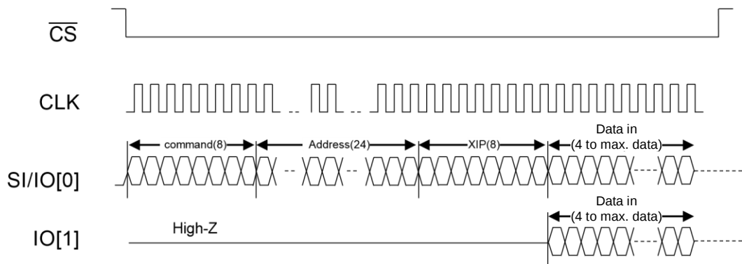
Figure 35 : Timing Description of 1-1-2 Instruction Type (Write with XIP)
