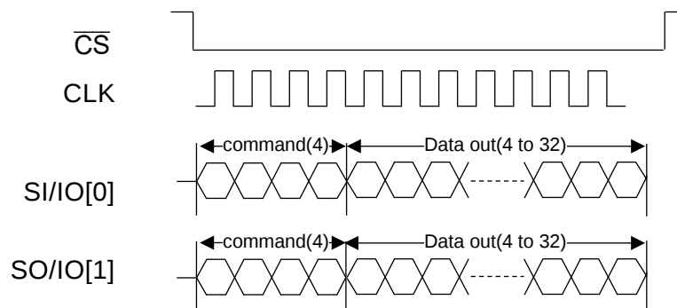
Figure 43 : Timing Description of 2-0-2 Instruction Type (Read)
