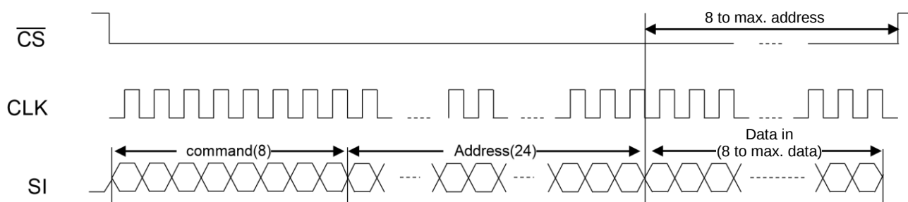
Figure 27 : Timing Description of 1-1-1 Instruction Type (Write)
