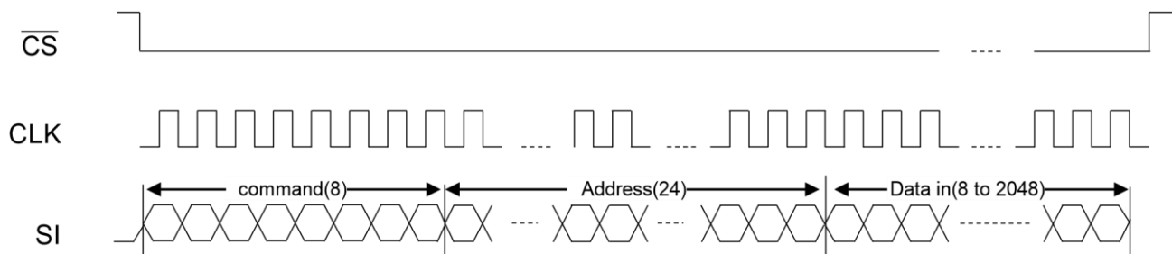
Figure 29 : Timing Description of 1-1-1 Augmented 256-byte Area (Write)
