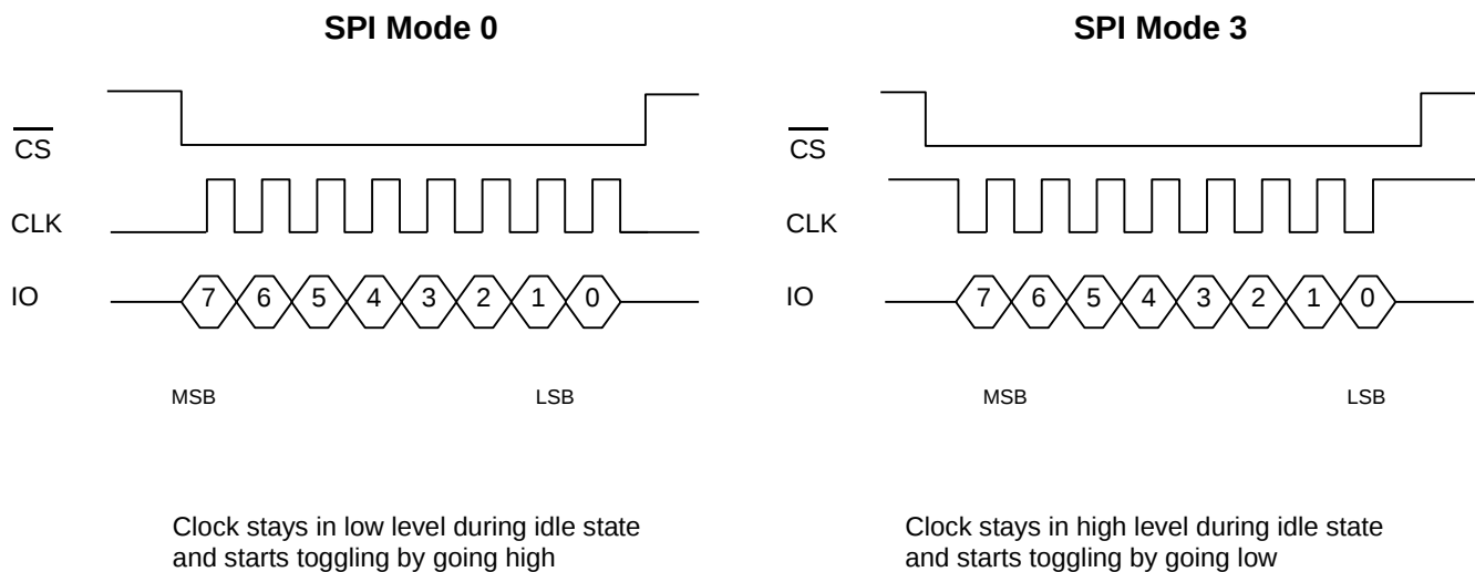
Figure 4 : SPI Clock Modes
