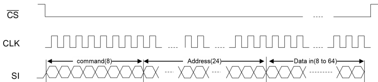
Figure 31 : Timing Description of 1-1-1 Any Register Instruction Type (Write)
