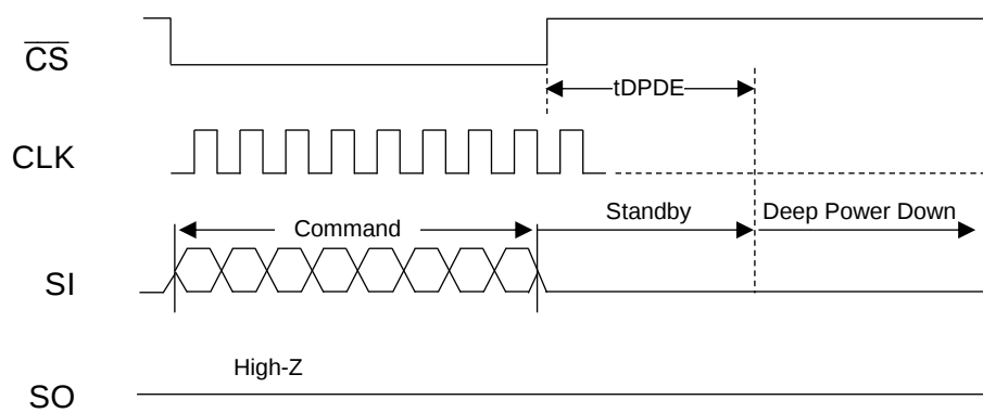
Figure 14 : Entering Deep Power Down Mode (SSIP mode)
