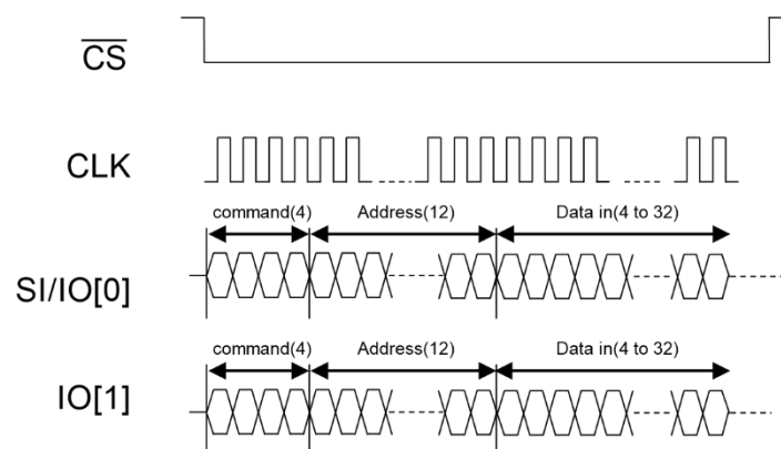
Figure 46 : Timing Description of 2-2-2 Any Register Instruction Type (Write)
