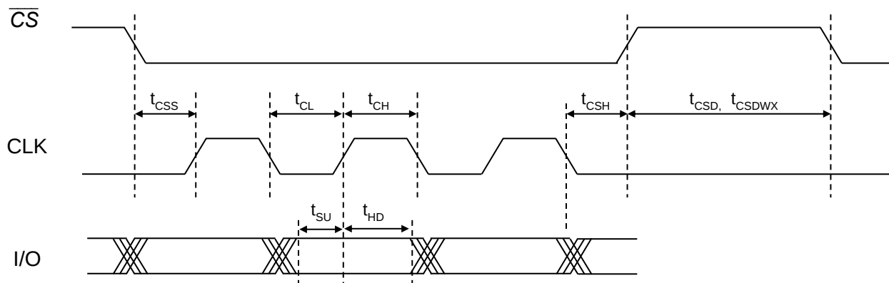
Figure 19 : Synchronous Input Timing (SDR)
