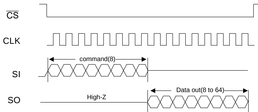
Figure 24 : Timing Description of 1-0-1 Instruction Type (Read)
