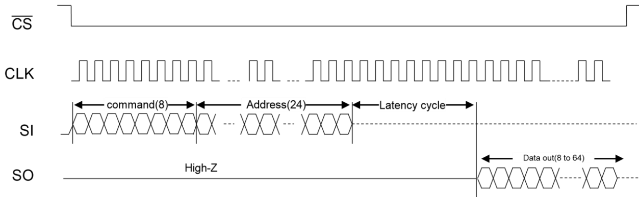
Figure 30 : Timing Description of 1-1-1 Any Register Instruction Type (Read)
