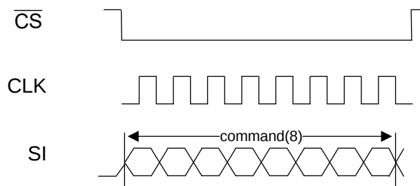
Figure 23 : Timing Description of 1-0-0 Instruction Type
