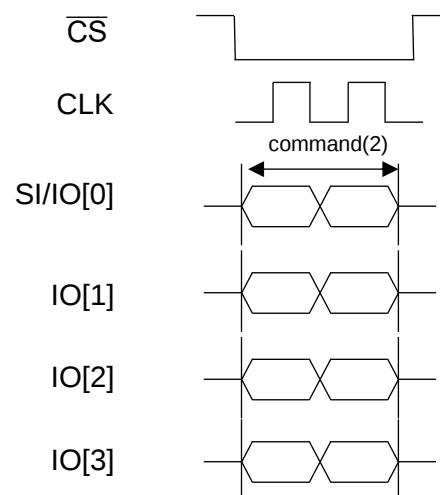
Figure 49 : Timing Description of 4-0-0 Instruction Type
