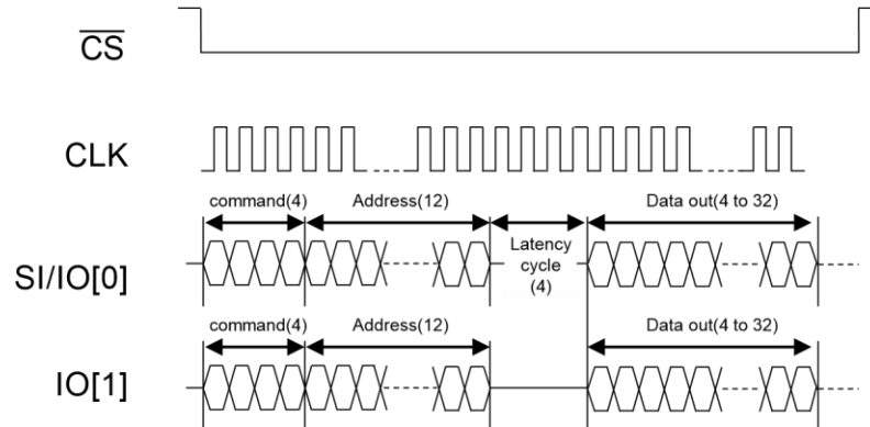
Figure 45 : Timing Description of 2-2-2 Any Register Instruction Type (Read)
