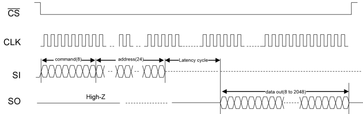
Figure 28 : Timing Description of 1-1-1 Augmented 256-byte Area (Read)
