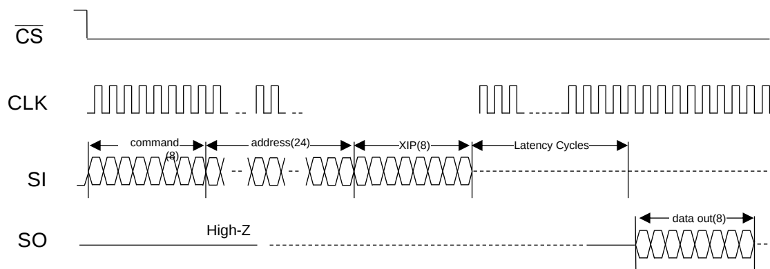
Figure 11 : Description of Read Operation with XIP (SSIP mode)
