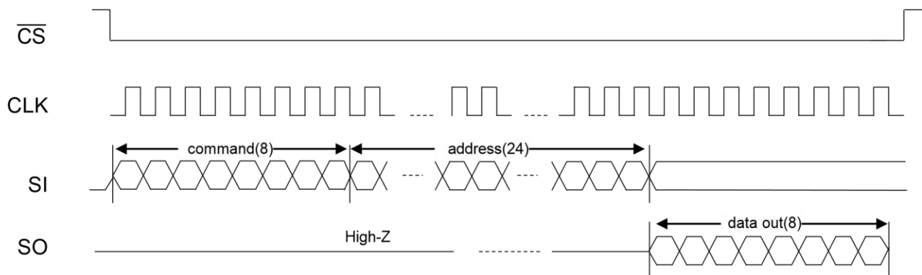
Figure 9 : Description of Read Operation (SSIP mode)
