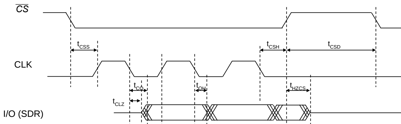
Figure 20 : Synchronous Data Output Timing (SDR)
