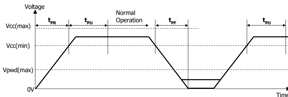
Figure 3 : Power-up/down Behavior
