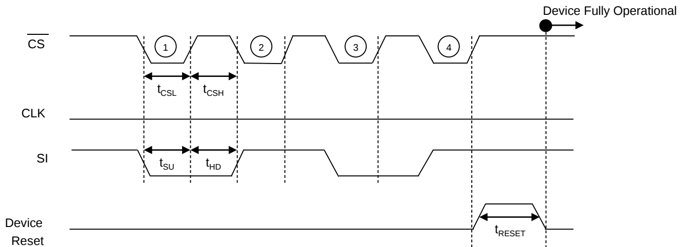
Figure 18 : JEDEC Reset Operation Timing
