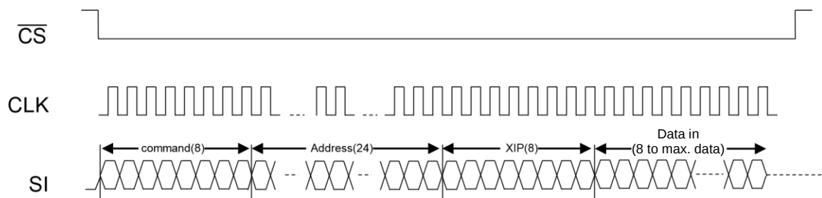
Figure 33 : Timing Description of 1-1-1 Instruction Type (Write with XIP)
