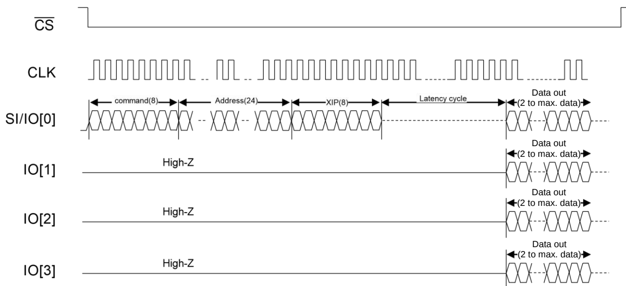
Figure 38 : Timing Description of 1-1-4 Instruction Type (Read with XIP)
