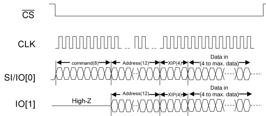
Figure 37 : Timing Description of 1-2-2 Instruction Type (Write with XIP)
