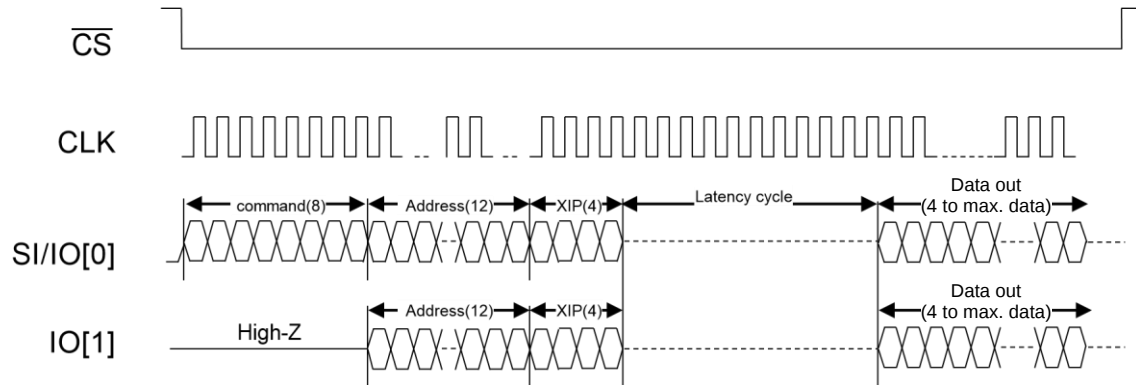
Figure 36 : Timing Description of 1-2-2 Instruction Type (Read with XIP)
