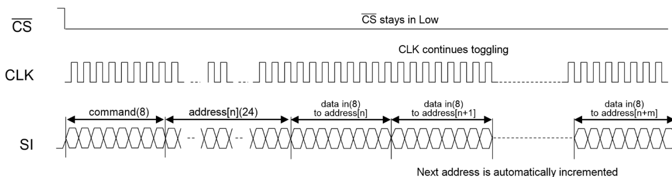
Figure 13 : Description of Continuing Write Operation (SSIP mode)
