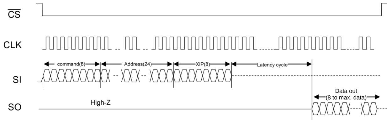
Figure 32 : Timing Description of 1-1-1 Instruction Type (Read with XIP)
