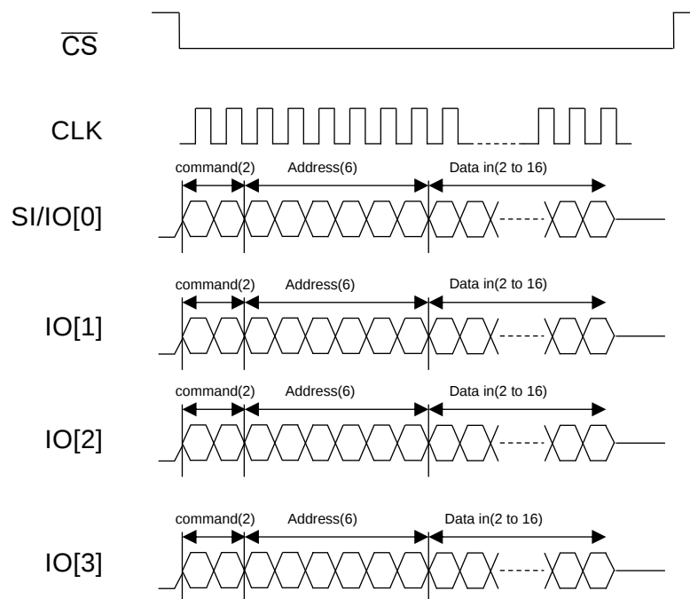
Figure 53 : Timing Description of 4-4-4 Any Register Instruction Type (Write)
