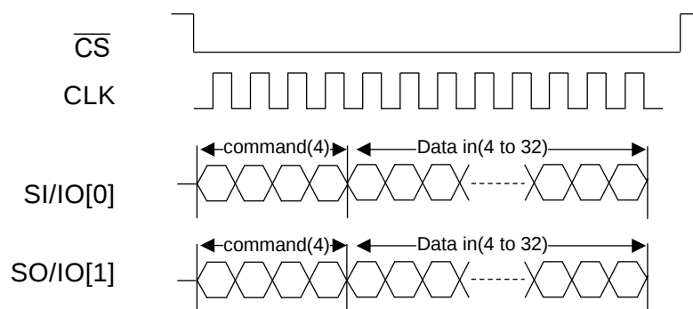
Figure 44 : Timing Description of 2-0-2 Instruction Type (Write)
