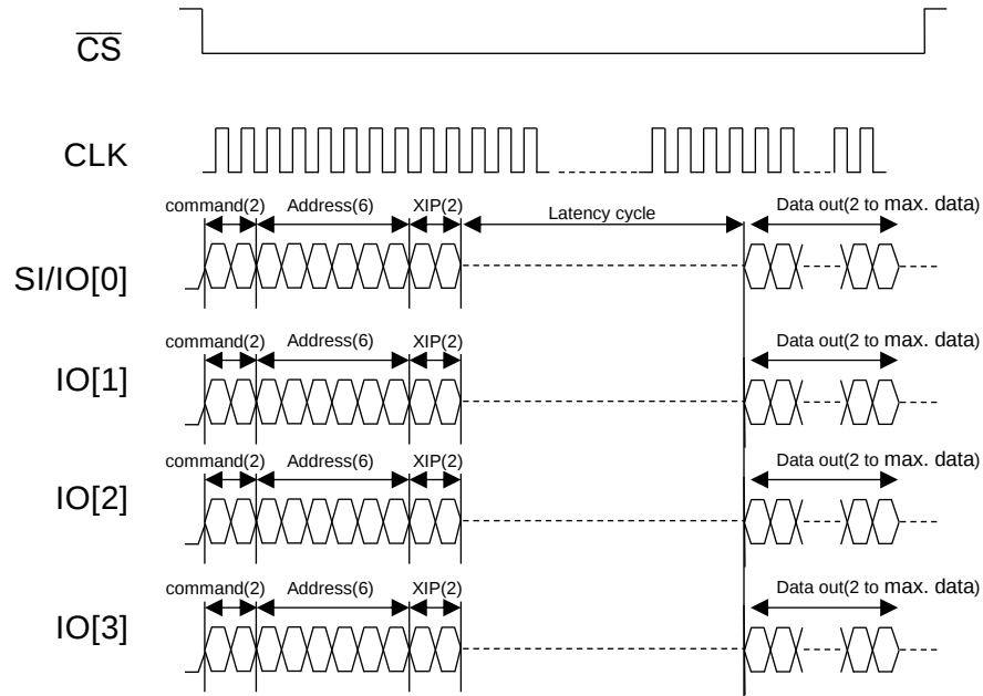
Figure 54 : Timing Description of 4-4-4 Instruction Type (Read with XIP)
