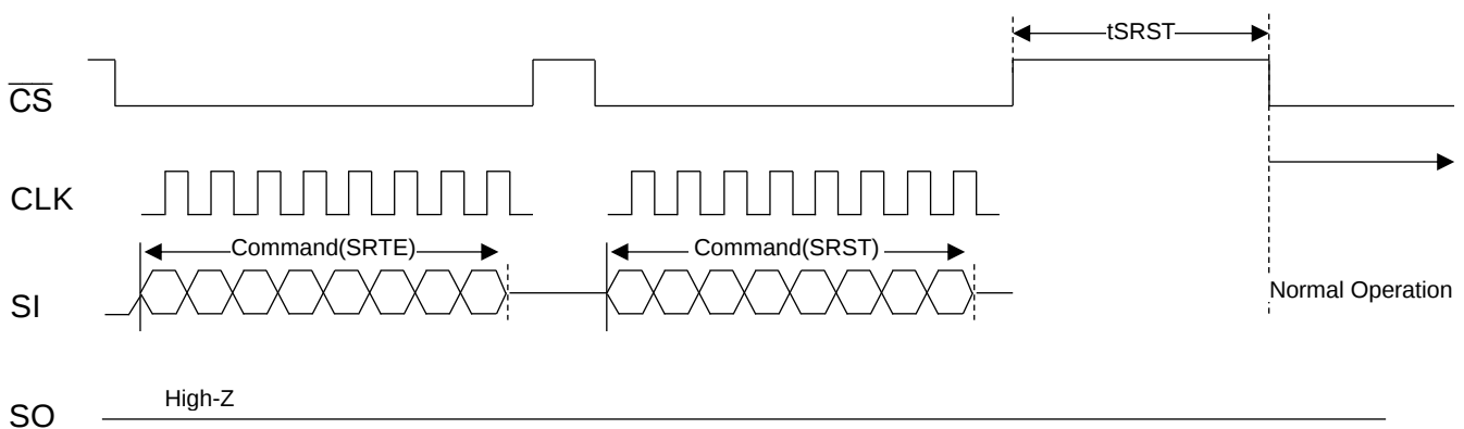
Figure 17 : Software Reset Timing
