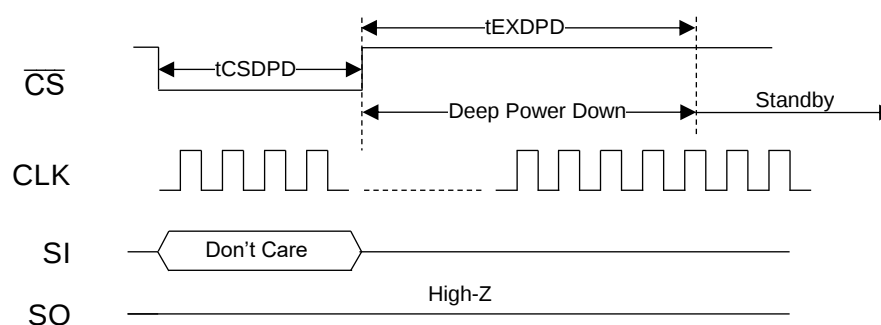
Figure 15 : Exit Deep Power Down Mode by \overline{CS}
