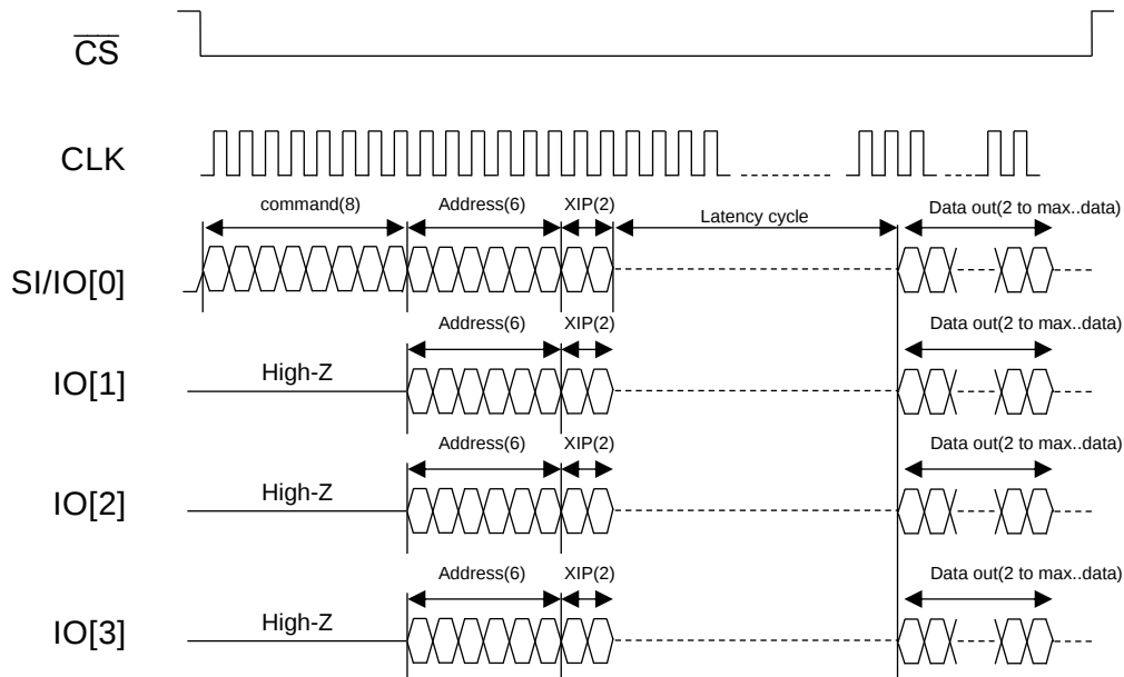
Figure 40 : Timing Description of 1-4-4 Instruction Type (Read with XIP)
