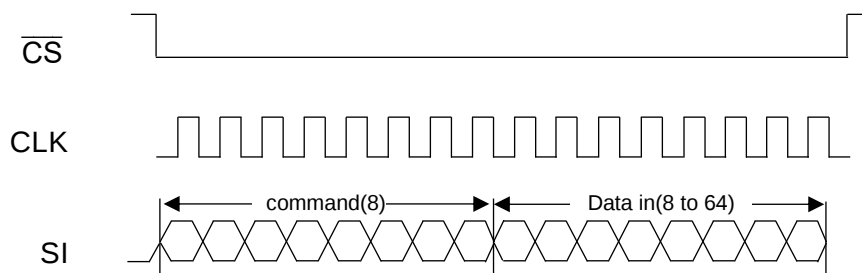
Figure 25 : Timing Description of 1-0-1 Instruction Type (Write)
