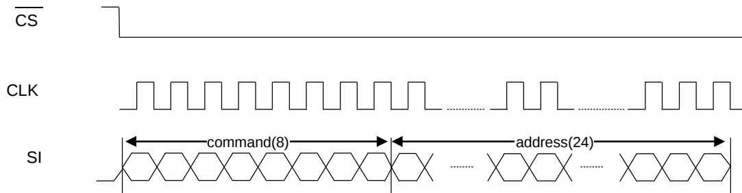
Figure 8 : Description of command followed by Address (SSIP mode)
