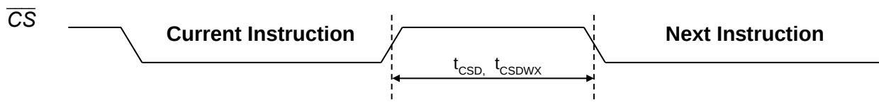
Figure 22 : \overline{\text{CS}} High Timing
