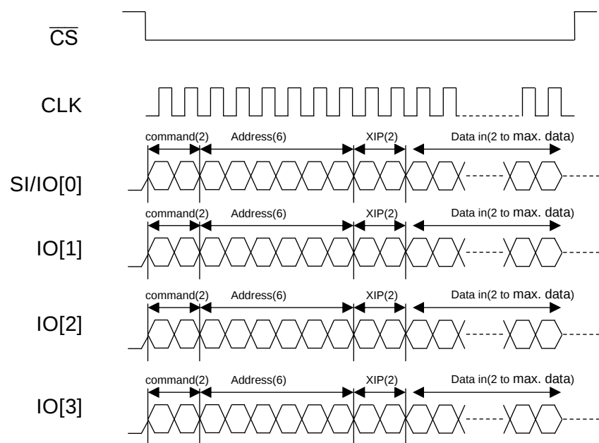
Figure 55 : Timing Description of 4-4-4 Instruction Type (Write with XIP)
