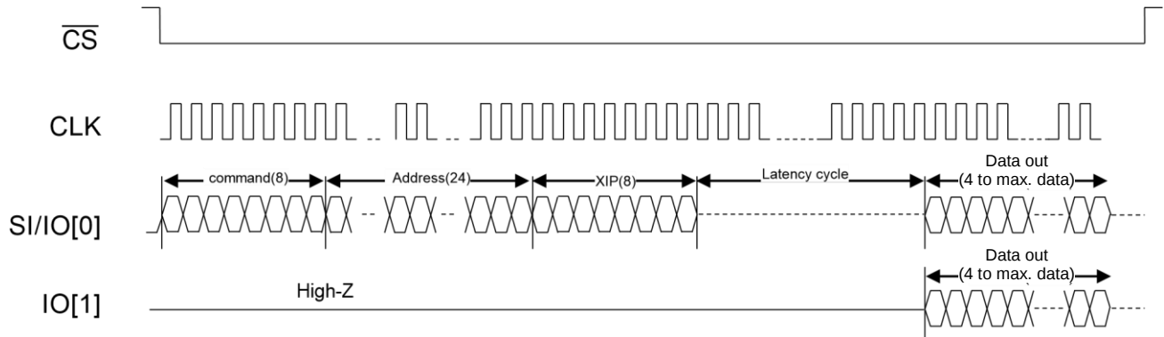
Figure 34 : Timing Description of 1-1-2 Instruction Type (Read with XIP)
