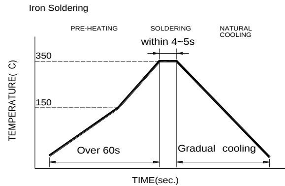
Fig.2 Iron soldering temperature profiles
