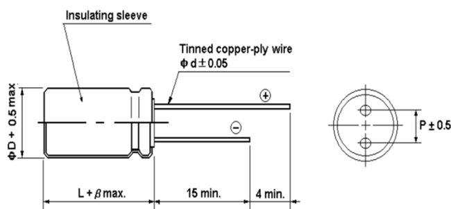
Dimensions of \phi D & L
