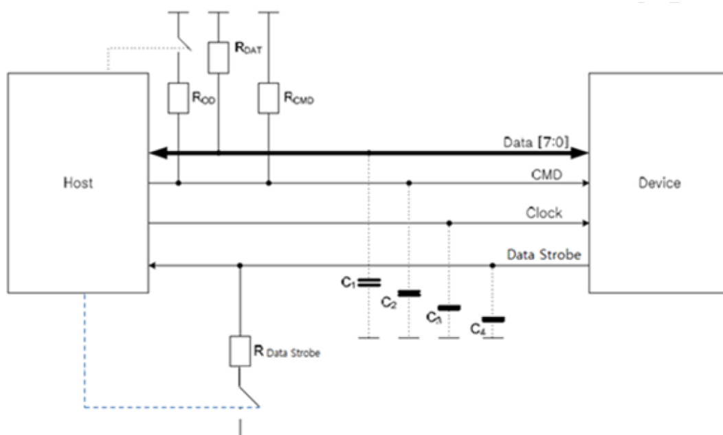
Figure 5 – Bus Circuitry Diagram
