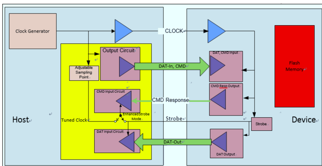
Figure 4 – HS400 Block Diagram
