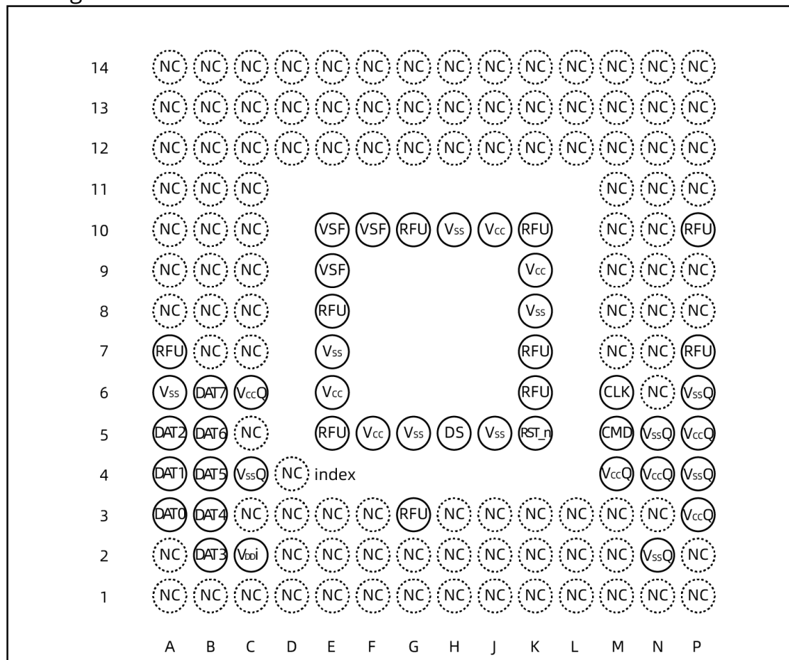
Figure 20 – Ball Assignment (Top View)
