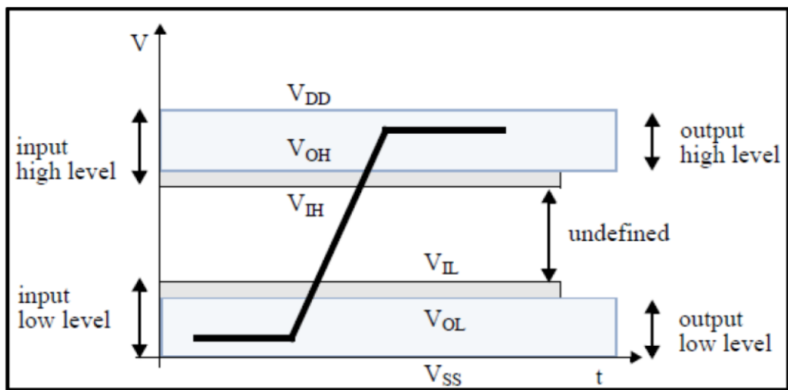
Figure 10 – Bus Signal Levels
