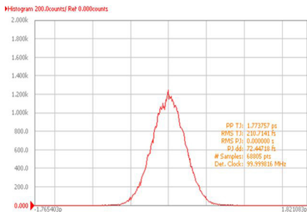
Frequency - 100.000MHz
