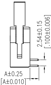
Short Latch
