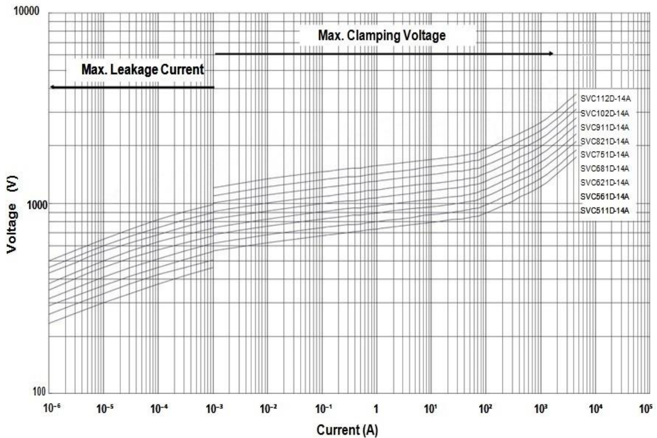
Fig 5-2) Example of transient V-I characteristic curves. Ø14
