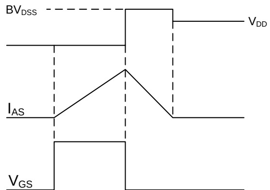
Fig.8 EAS Waveform
