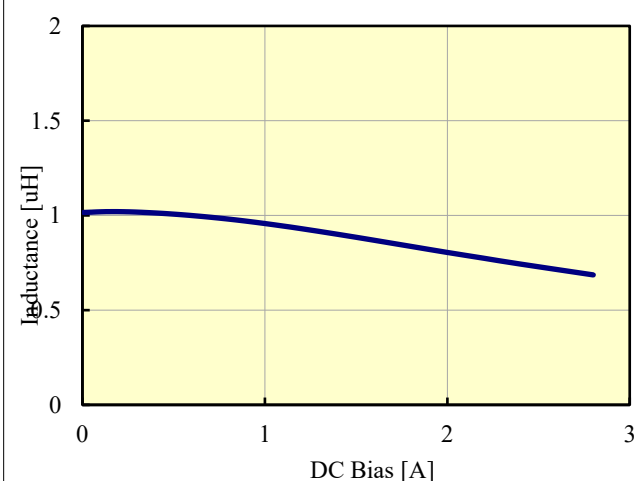
DC Bias vs Inductance
