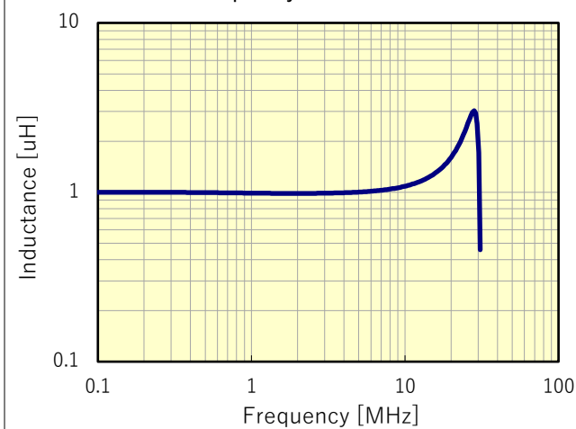
Frequency vs Inductance
