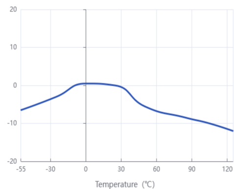
Capacitance-Temperature Characteristics
