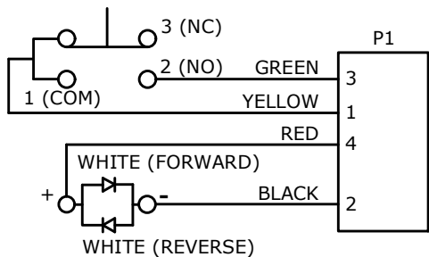
SCHEMATIC SPDT - ON - (ON) ILLUMINATED ( ) DENOTES MOMENTARY
