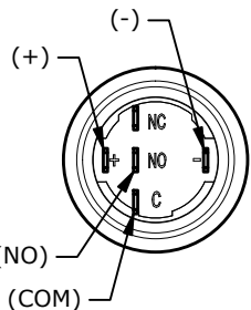
BOTTOM VIEW SHOWN WITHOUT WIRING AND CONNECTOR
